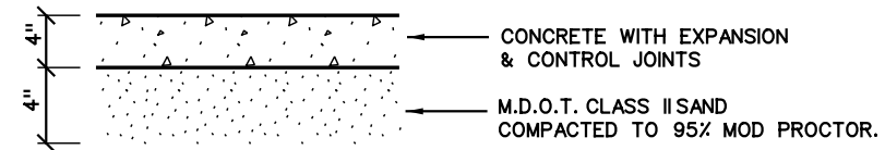
TYPICAL 4" CONCRETE SIDEWALK
