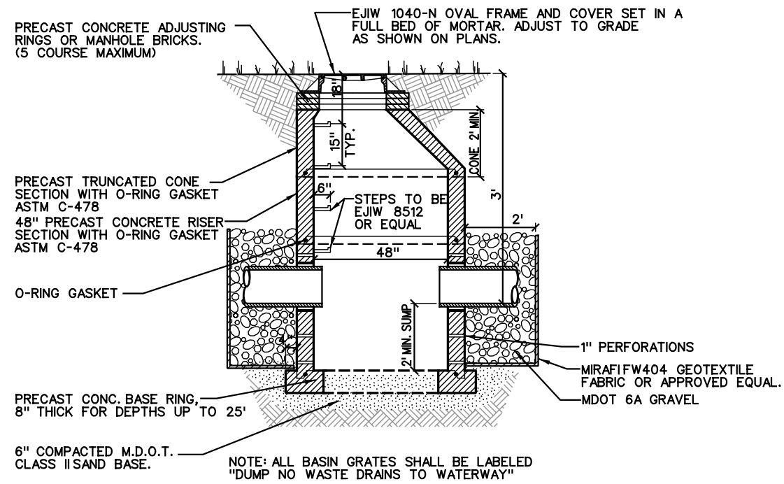
STORM SEWER FOUR FOOT DIAMETER LEACHING BASIN
